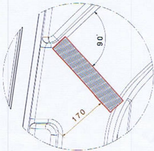
Detail 05
