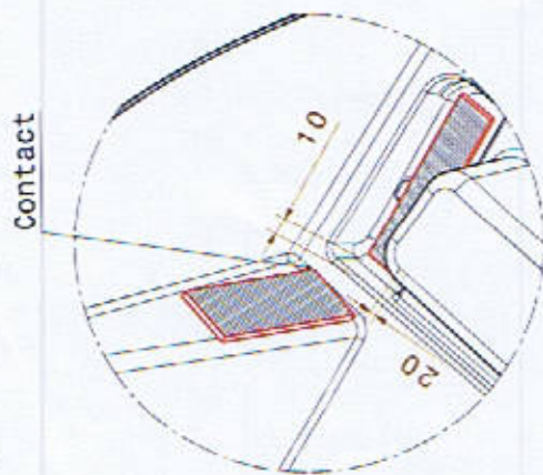
Detail 17
